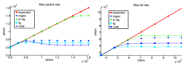
Figure 1: Generated packet- and bit-rate.
