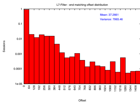
Fig. 2: Distribution of the offset of a matching string inside its last packet.
