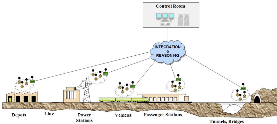
Fig. 3. SENSORAIL architecture
