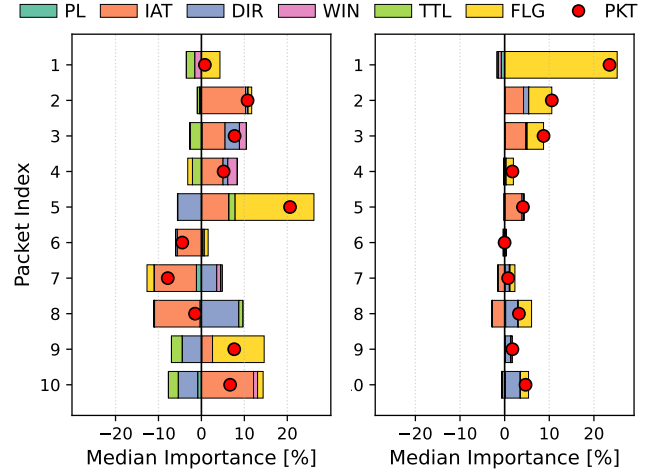
Fig. 3: Explainability results for the Benign class: comparison between CNN (left) and LSTM (right). Per-packet importance is obtained by aggregating per-feature contributions.
