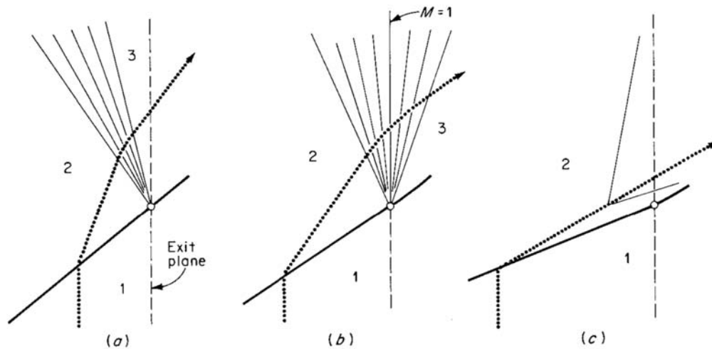
Com Figure 8.38 Shock incident on an open end.
