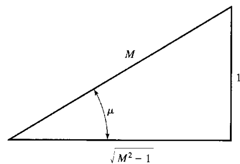
Figure 14.4 Mach Triangle
