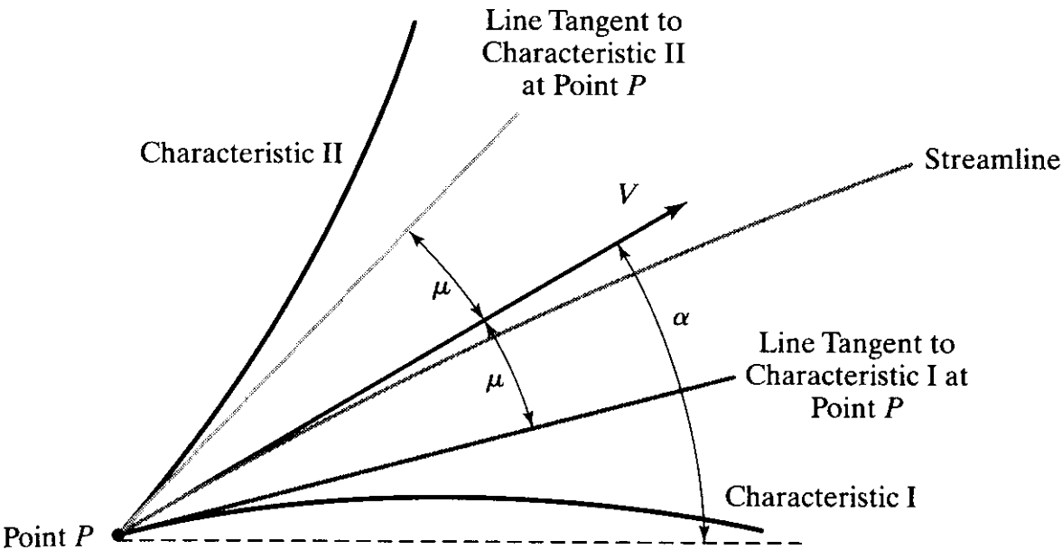
Figure 14.5 Geometry of Characteristics at a Point
