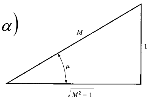
Figure 14.4 Mach Triangle
