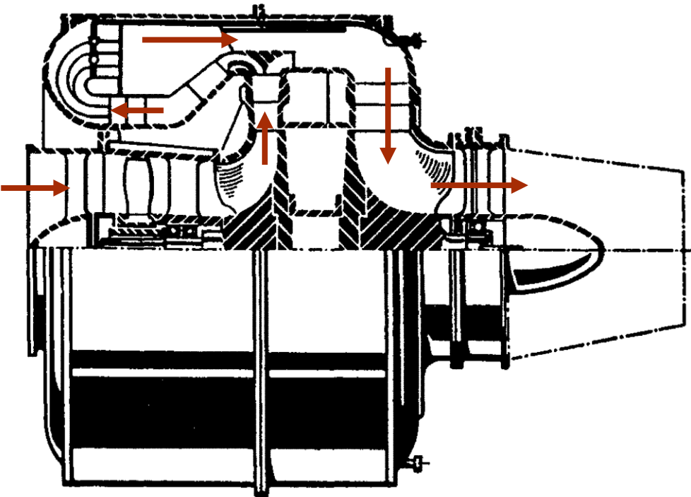
Fig. 12 1937 design of the He.S3 turbojet engine.
