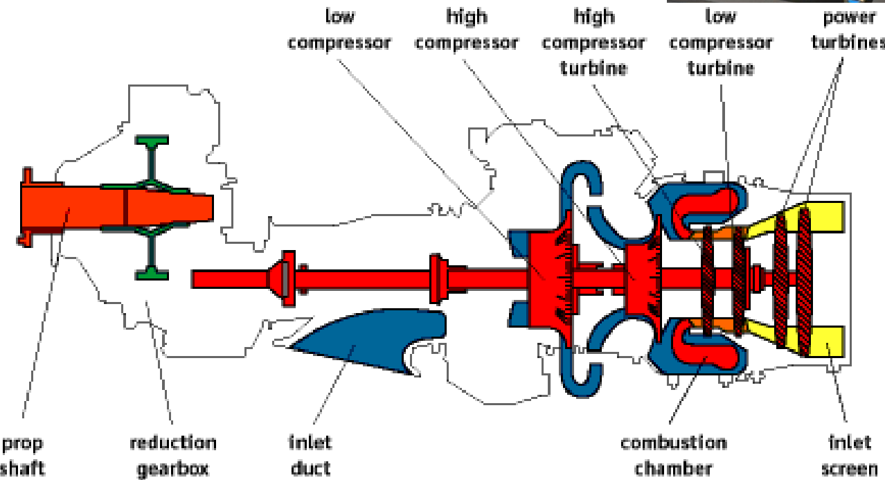
PW127 (ATR). Peso 500kg, L=2.1m , D=.85m , Equivalent Power 2200kW, Comp 1/1, Turb 1/1/2.
