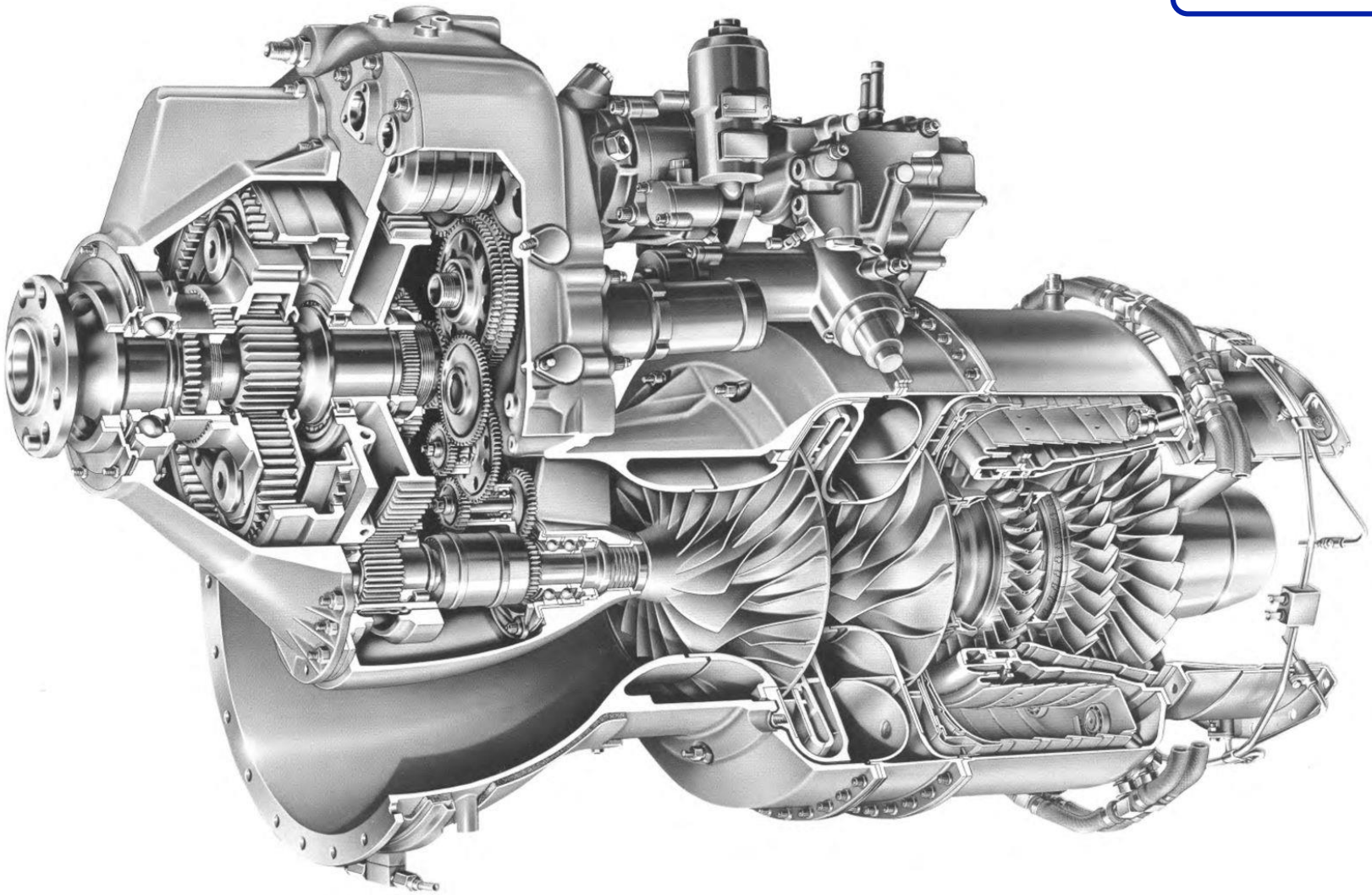
Garrett TPE331. Peso 175kg, L=1.1m , D=.53m , Equivalent Power 700kW, Comp 2, Turb 3.
