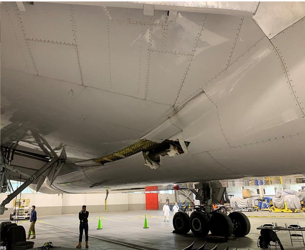
PW 4000 (777). Peso 7000kg, L=4.8m , D=2.84m , F_{max}=420kN , \alpha=6 , \pi_c=50 , Comp 1/7/11, Turb 2/7. Incidente del 20.2.2021
