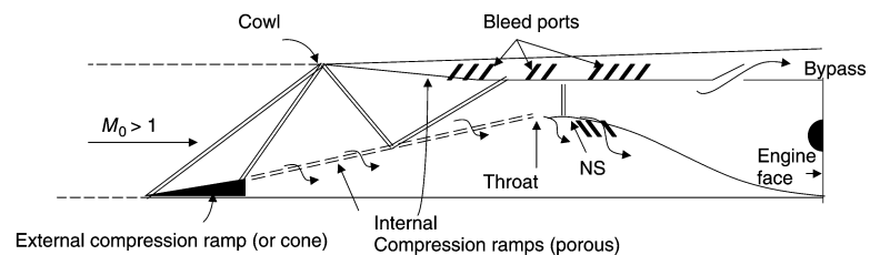
(a) The oblique shock is at the lip and the cowl shock causes external (wave) drag
