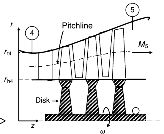
(b) Constant hub radius
