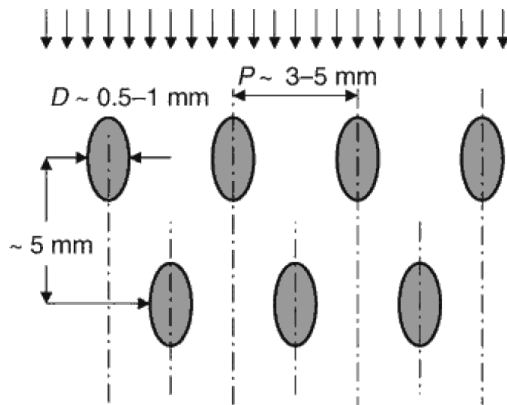
(a) Geometry of a staggered array
