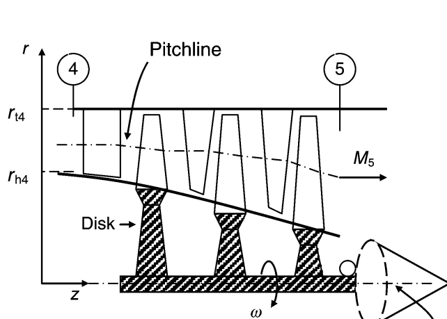
(a) Constant tip radius
