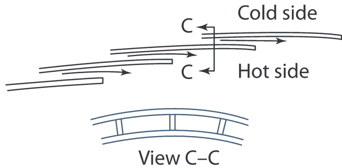
b) Convection/film-cooled liner
