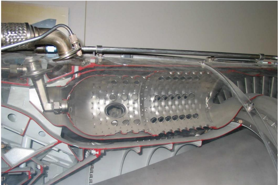
a) Louver-cooled liner
