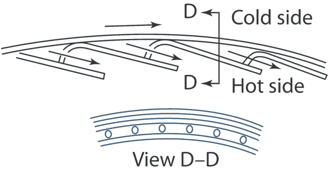
d) Impingement/film-cooled liner
