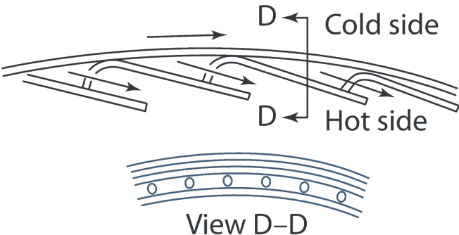
d) Impingement/film-cooled liner
