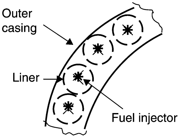
(a) Can-annular combustor
