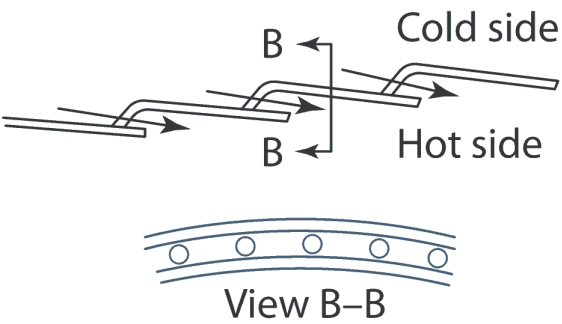
c) Film-cooled liner
