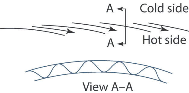
a) Louver-cooled liner
