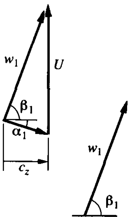
(a) Positive incidence flow separation
