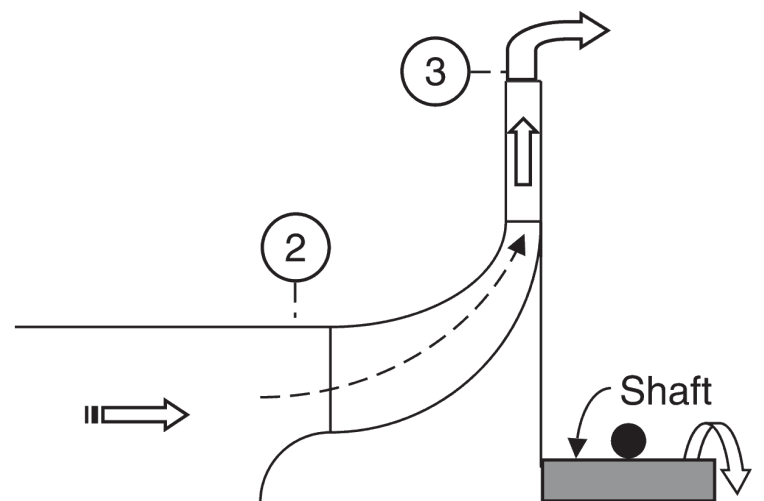
(b) A radial-flow or centrifugal compressor
