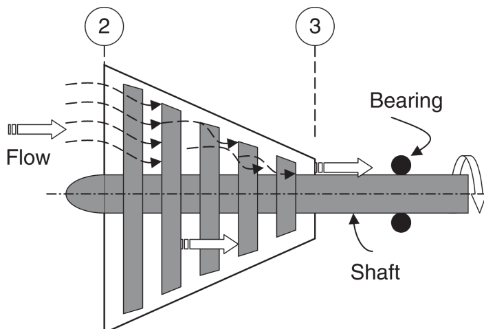
(a) An axial-flow compressor
