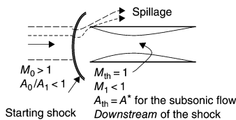
(d) At supersonic Mach numbers a starting (bow) shock is formed in front of the inlet causing spillage drag while the throat remains choked
