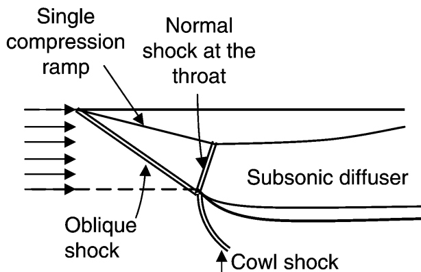
(a) A single compression ramp inlet involves one oblique shock and one normal shock
