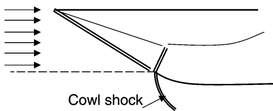
(a) The oblique shock is at the lip and the cowl shock causes external (wave) drag
