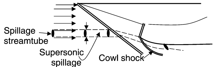
(b) The oblique shock is projected below the cowl lip creating some supersonic spillage flow but cowl shock is now weaker causing lower external drag
