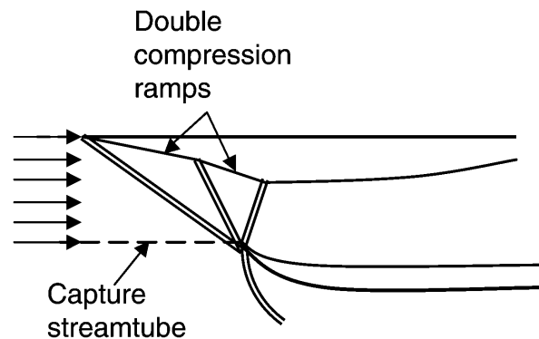
(b) A double compression ramp inlet creates two oblique shocks and one NS
