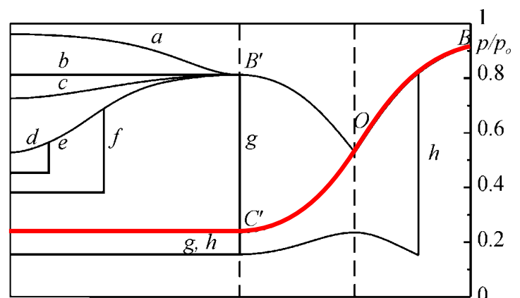
(d) At supersonic Mach numbers a starting (bow) shock is formed in front of the inlet causing spillage drag while the throat remains choked
