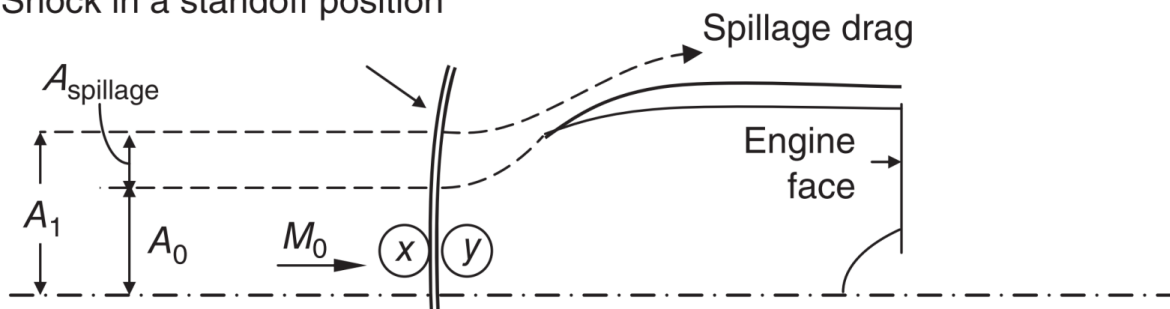
(a) Normal shock inlet in subcritical mode (high backpressure—low m and m_{\text{cor}} )
