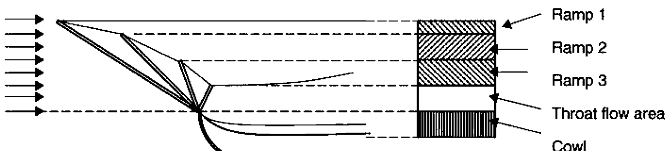
(c) The side view of a three-compression ramp inlet with three oblique shocks and one normal shock
