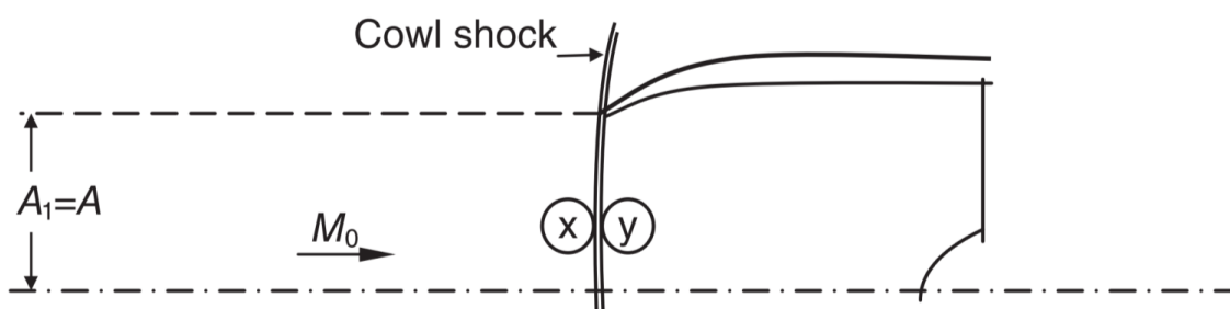
(b) Normal shock inlet in critical mode (low backpressure— \dot{m}_{\text{Design}} )
