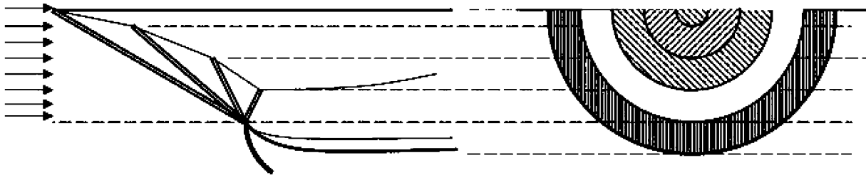
(e) A three-cone external compression inlet shows three conical shocks and one NS
