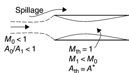
(c) At higher subsonic Mach numbers than (b) the capture ratio falls below 1 and spillage occurs (note the throat remains choked)
