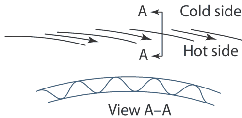
a) Louver-cooled liner
