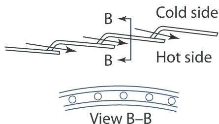
c) Film-cooled liner
