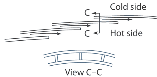
b) Convection/film-cooled liner
