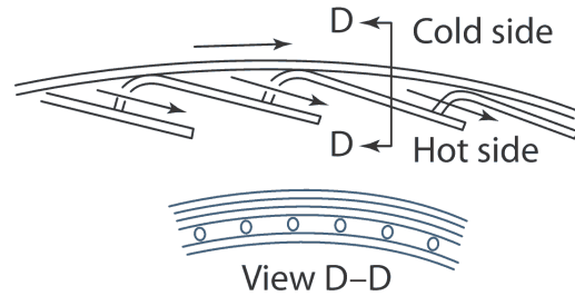
d) Impingement/film-cooled liner
