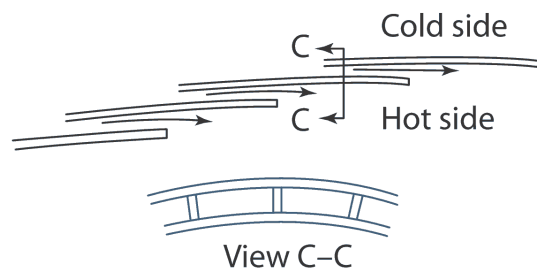
b) Convection/film-cooled liner
