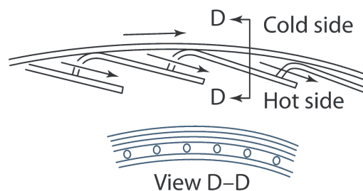
d) Impingement/film-cooled liner
