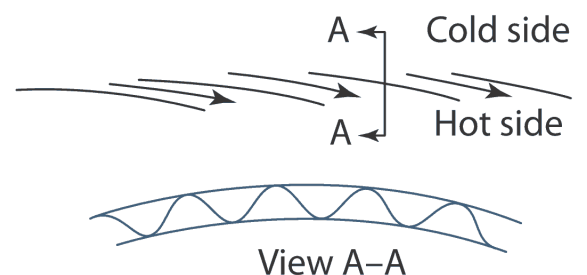
a) Louver-cooled liner
