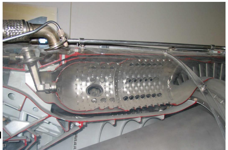
CROSS-IGNITION TUBE AND CLAMP
