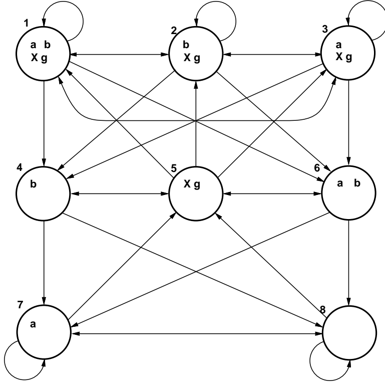
Figure 1: Tableau for a \mathbf{U} b
