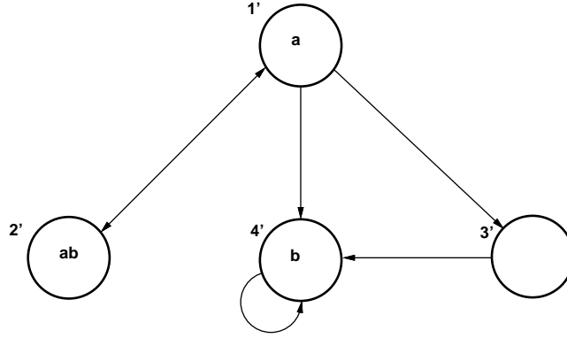
Figure 2: Kripke Structure M
