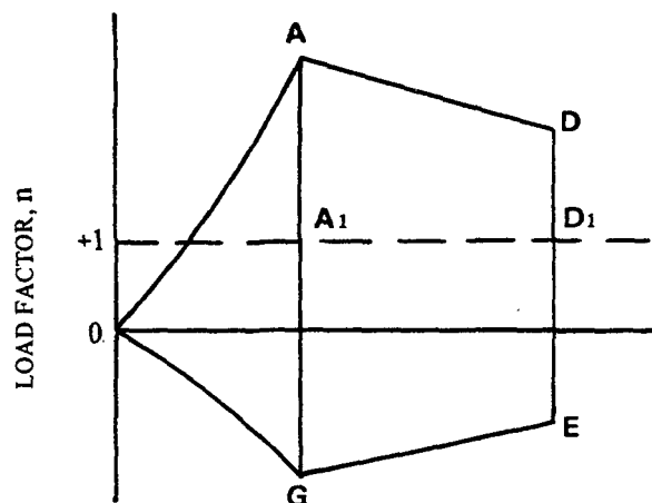
FIGURE 1 PITCHING MANOEUVRES
