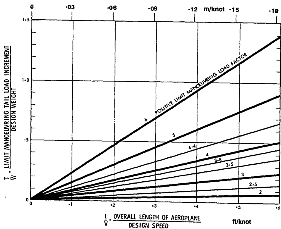
FIGURE B2 — MANOEUVRING TAIL LOAD INCREMENT (UP OR DOWN).
