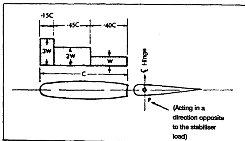
FIGURE B6 — TAIL SURFACE LOAD DISTRIBUTION.
