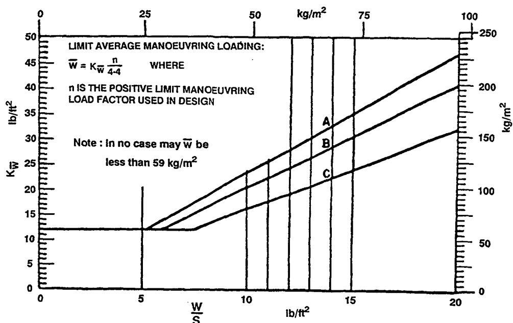
FIGURE B1 — LIMIT AVERAGE MANOEUVRING CONTROL SURFACE LOADING.
