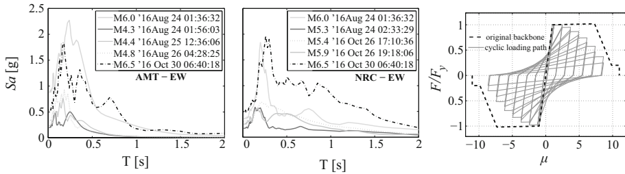
Fig. 8 Pseudo-acceleration response spectra of the five shocks considered in the illustrative analysis of cumulative damage during the sequence at Amatrice (left) and Norcia (center). Backbone curve and cyclic loading hysteresis of the case-study SDOF systems (right)
