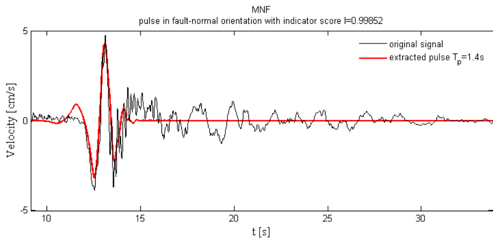
Figure 10.5 Original velocity time-history and CWT extracted pulse and residual signal for the fault-normal component of the Fiastra record - 24/08/2016 M_w 6.0 event.
