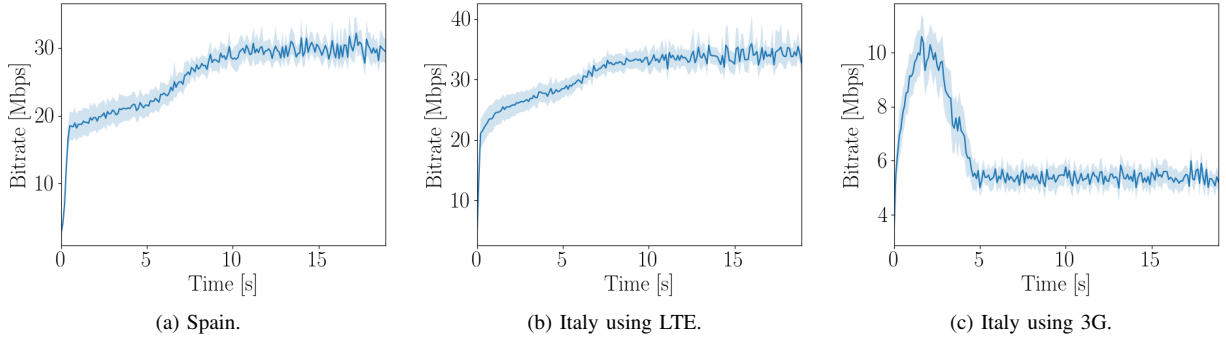
Fig. 2: Time series for TCP achievable throughput. Observations from all experiments, time is calculated since the beginning of the experiment. Shaded area represents 95 th percentile bootstrapped confidence interval.
