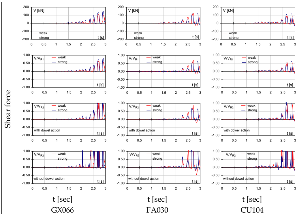
Figure 7.32. Analysis results for the top of column #3 (shear force and demand over capacity ratios for conventional shear V_{R1} , for sliding shear V_{R2} with and without dowel action).
