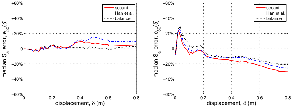
Figure 5.30. The relative error in the median S_a -capacity of the secant, Han et al and balanced fits for T = 0.2 s, when applied to the capacity curves of Figure 5.29: (a) step-mild versus (b) mild-steep trend in the softening slope.
