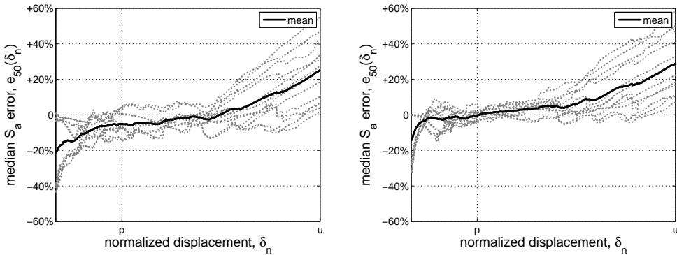
Figure 5.28. The mean of the relative error in the median S_a -capacity for (a) the 60%L and (b) 10%H fits, applied to the capacity curves of Figure 19b, for T = 2.0 s.
