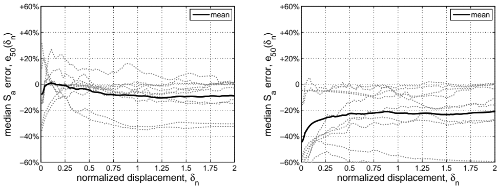
Figure 5.10. The mean of the relative error in the median S_a -capacity for (a) the 10% fit and (b) the 60% fit, for a reference period of T = 0.5 s and for ten generalized elastic-plastic systems, represented by the grey dotted lines.
