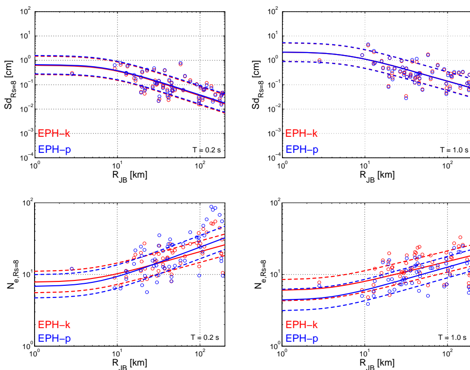
Figure 2.13. Estimates for a magnitude 6.0 earthquake, soil type A and R_s equal to 8 at two natural periods ( T=0.2s and 1.0s ) for both EPH-k and EPH-p systems, plotted as a function of R_{JB} and compared with Sd_i and N_e data for a magnitude interval of 6.0\pm 0.3 .
