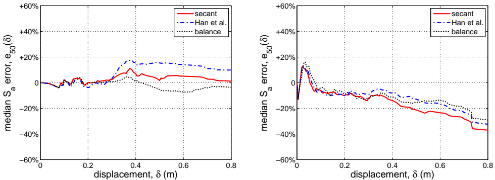
Figure 5.31. The relative error in the median S_a -capacity of the secant, Han et al and balanced fits for T = 0.5 s, when applied to the capacity curves of Figure 5.29: (a) step-mild versus (b) mild-steep trend in the softening slope.
