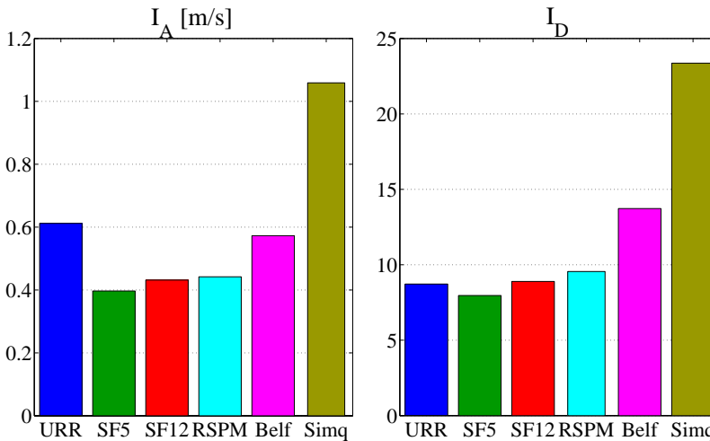
Figure 3.2. Average values of I_A and I_D for the considered classes of records.
