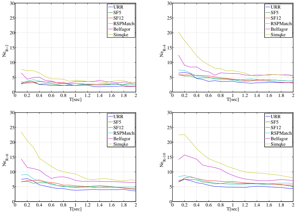
Figure 3.9. Average values of equivalent number of cycles for EPH system computed as mean value of 28 records.
