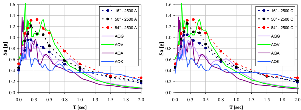
Figure C.11. Comparison of spectra of the four signals registered within 15km and UHS acceleration spectra evaluated for three different percentiles ( 16^\circ , 50^\circ and 84^\circ ) on A soil class (a) and C soil class (b) for T_r equal to 2500 years.
