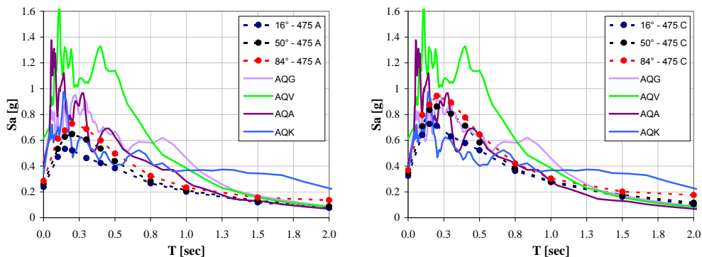
Figure C.10. Comparison of spectra of the four signals registered within 15km and UHS acceleration spectra evaluated for three different percentiles ( 16^\circ , 50^\circ and 84^\circ ) on A soil class (a) and C soil class (b) for T_r equal to 475 years.
