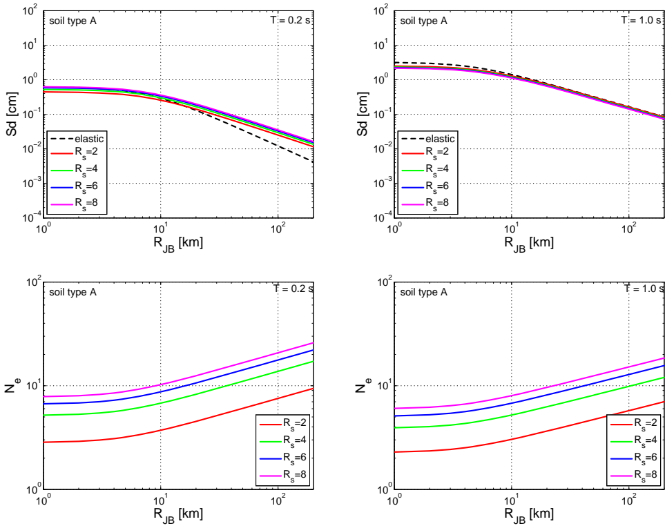
Figure 2.18. Predictions of S_{di} and N_e for EPH-k SDOF systems at the different R_s values, M_w equal to 6.0 and soil class A, for T = 0.2 s and 1.0 s.
