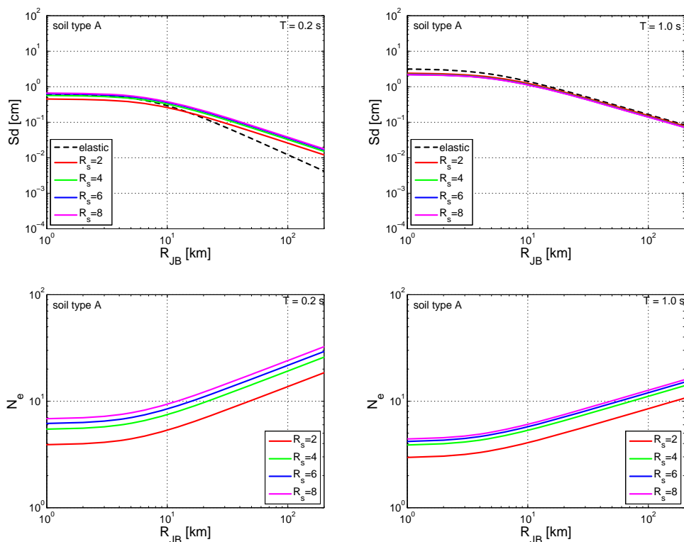
Figure 2.19. Predictions of S_{di} and N_e for EPH-k SDOF systems at the different R_s values, M_w equal to 6.0 and soil class A, for T = 0.2 s and 1.0 s.
