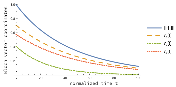
Fig. 13. Combined y-z-phase damping: time-domain evolution of a qubit subject to the Hamiltonian H_s = \Omega\sigma_z/2 , when emerging from initial pure state of |\psi(0)\rangle = \sqrt{\frac{1+\sqrt{3}}{2\sqrt{3}}}|0\rangle + \frac{i+\sqrt{3}}{2\sqrt{3+\sqrt{3}}}|1\rangle located at the Bloch vector coordinates \mathbf{r}(0) = [\frac{1}{\sqrt{2}}, \frac{1}{\sqrt{6}}, \frac{1}{\sqrt{3}}] . Left plot: representation of the qubit's time evolution with respect to the Bloch sphere. Right plot: Bloch vector coordinates \mathbf{r}(t) as a function of time, with the phase evolution engendered by the energy difference \Omega in H_s appropriately compensated, as detailed in the text.
