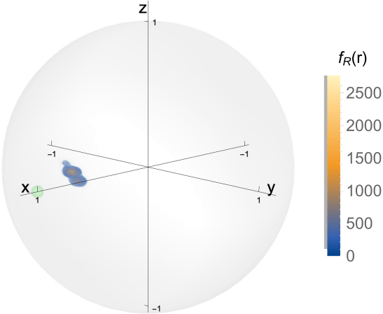
Fig. 17. Teleportation with 5-qubits IBM Tenerife ibmqx4 quantum processor between chip-qubits q[0] and q[2] . Initial pure state |\psi\rangle = |+\rangle with Bloch vector coordinates \mathbf{r} = [1, 0, 0] (green dot in Fig. 17d).
