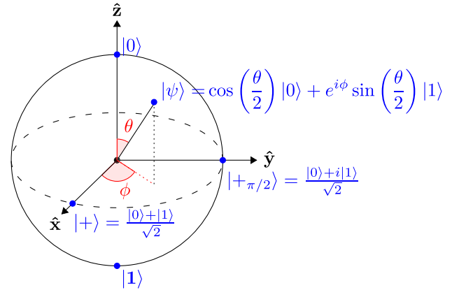
Fig. 1. Bloch sphere: geometrical representation of a qubit in spherical coordinates. A pure state |\psi\rangle = \alpha|0\rangle + \beta|1\rangle is represented by a point on the sphere surface, with \alpha = \cos \frac{\theta}{2} and \beta = e^{i\phi} \sin \frac{\theta}{2} .
