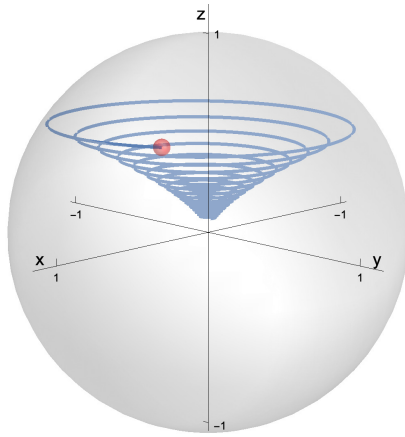
Fig. 13. Combined y-z-phase damping: time-domain evolution of a qubit subject to the Hamiltonian H_s = \Omega\sigma_z/2 , when emerging from initial pure state of |\psi(0)\rangle = \sqrt{\frac{1+\sqrt{3}}{2\sqrt{3}}}|0\rangle + \frac{i+\sqrt{3}}{2\sqrt{3+\sqrt{3}}}|1\rangle located at the Bloch vector coordinates \mathbf{r}(0) = [\frac{1}{\sqrt{2}}, \frac{1}{\sqrt{6}}, \frac{1}{\sqrt{3}}] . Left plot: representation of the qubit's time evolution with respect to the Bloch sphere. Right plot: Bloch vector coordinates \mathbf{r}(t) as a function of time, with the phase evolution engendered by the energy difference \Omega in H_s appropriately compensated, as detailed in the text.
