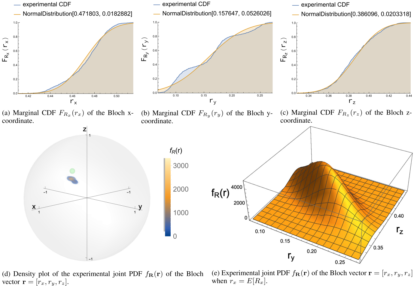
Fig. 18. Teleportation with 5-qubits IBM Tenerife ibmqx4 quantum processor between chip-qubits q[0] and q[2] . Initial pure state |\psi\rangle = \sqrt{\frac{1+\sqrt{3}}{2\sqrt{3}}}|0\rangle + \frac{i+\sqrt{3}}{2\sqrt{3+\sqrt{3}}}|1\rangle with Bloch vector coordinates \mathbf{r} = [\frac{1}{\sqrt{2}}, \frac{1}{\sqrt{6}}, \frac{1}{\sqrt{3}}] (green dot in Fig. 18d).
