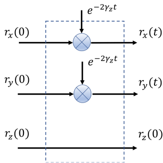
Fig. 10. Phase-Damping model.
