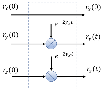
Fig. 12. y-z damping model.
