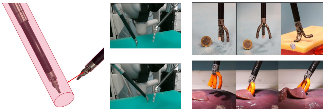
Figure 8: Left: A marker-less method tracks surgical tools, establishing VF geometry resembling to a cylinder with its central axis aligned with the instrument's axis [102]; Right: The MUSH Hand II surgical tool, integrated on the dVRK robot [94, 132, 145].
