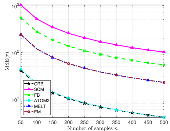
Figure 5: MSE vs. number of samples n for banded Toeplitz covariance matrix.
