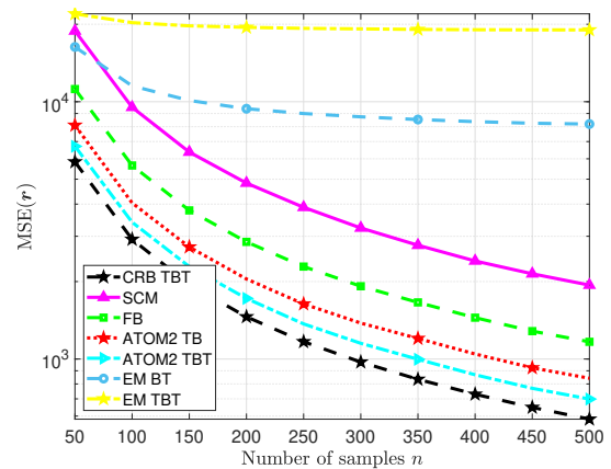
Figure 6: MSE vs. number of samples n for TBT covariance matrix.
