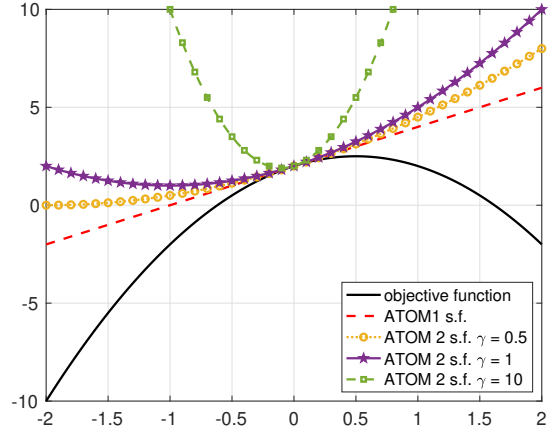
Figure 1: A notional representation of the objective function of Problem (10) and the corresponding s.f. of ATOM1 and ATOM2, with the latter employing \gamma \in \{0.5, 1, 10\} , for a one-dimensional optimization problem.
