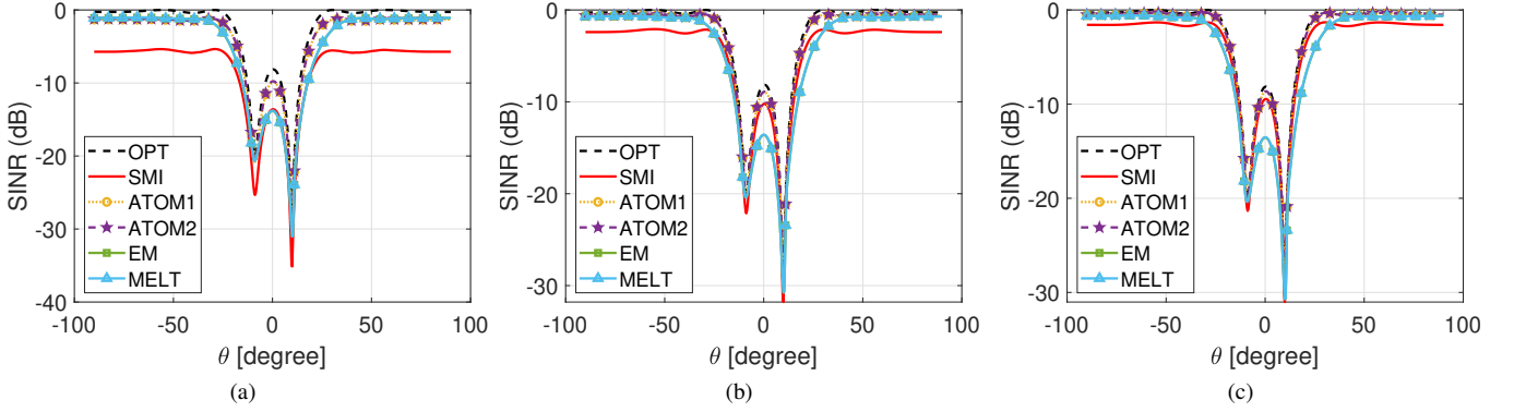
Figure 7: Average SINR vs \theta in the presence of two jammers, assuming m = 6 and a) n = m b) n = 2m , and c) n = 3m .
