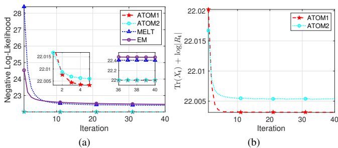
Figure 3: Negative log-likelihood (9) and the objective function of (10) vs. outer-iterations for m = 6 , n = 20 , and off-grid frequencies scenario.
