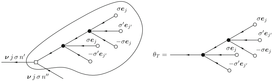
Fig. 11. An example of self-energy cluster T \in \mathfrak{E}_{j,\sigma,j,\sigma}^k(\omega \cdot \mathbf{v}, n) and the corresponding tree \theta_T . (Only the mode labels of the end nodes are shown in T and \theta_T .)
