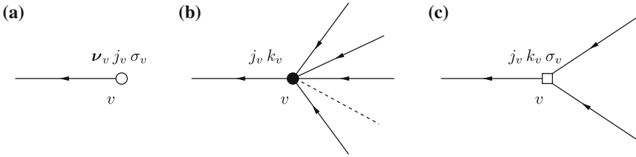
Fig. 2. Nodes and labels associated with the nodes: (a) end node v with s_v = 0 , j_v \in \{1, \dots, d\} , \sigma_v \in \{\pm\} , and \mathbf{v}_v = \sigma_v \mathbf{e}_{j_v} (cf. Sect. 3.3); (b) internal node v with s_v \geq 2 , j_v \in \{1, \dots, d\} , and k_v = s_v - 1 (cf. Sect. 3.3); (c) internal node v with s_v = 2 , j_v \in \{1, \dots, d\} , k_v = 0 , \sigma_v \in \{\pm\} (cf. Sect. 3.3)
