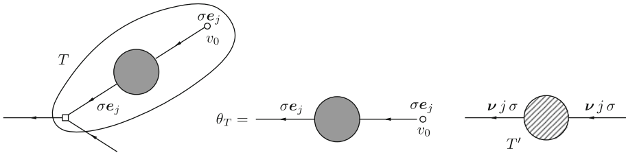
Fig. 15. The self-energy cluster $T$, the tree $\theta_T$, and the self-energy cluster $T'$ in the proof of Lemma 6.1
