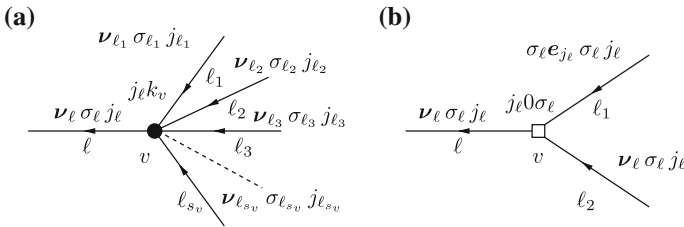
Fig. 5. Conservation law: (a) v with k_v = s_v - 1 \geq 1 , so that \nu_l = \nu_{l_1} + \dots + \nu_{l_{s_v}} , (b) v with s_v = 2 and k_v = 0 . (The scale labels are not shown)
