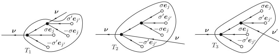
Fig. 16. The sets $\mathcal{F}_1(T) = \{T_1, T_2\}$ and $\mathcal{F}_2(T) = \{T_3\}$ corresponding to the self-energy cluster $T$ in Fig. 11
