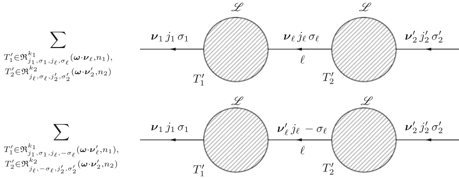
Fig. 18. Graphical representation of the cancellation mechanism discussed in the text: \mathbf{v}'_\ell = \mathbf{v}_\ell - 2\sigma_\ell e_{j_\ell} . If we sum the two contributions we obtain a gain factor O(2^{-n_\ell})
