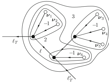
Fig. 8. Example of self-energy cluster: consider the cluster T on scale 3 in Fig. 7, and suppose that the mode labels of the end nodes are such that |\nu_1 + \nu_2 + \nu_3 + \nu_4 + \nu_5 + \nu_6| \leq 2 and \delta_{j_{\ell_T}}(\omega \cdot \nu_{\ell_T}) = \delta_{j_{\ell'_T}}(\omega \cdot \nu_{\ell'_T}) . Then T is a self-energy cluster with external lines \ell'_T (entering line) and \ell_T (exiting line). The path \mathcal{P}_T is such that \mathcal{P}_T = \{\ell\}
