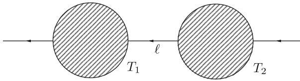
Fig. 9. Example of resonant line: \ell is resonant if both T_1 and T_2 are self-energy clusters
