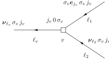
Fig. 4. If there is an internal node v with k_v = 0 then s_v = 2 and the following constraints are imposed on the other labels: \sigma_{l_v} = \sigma_{l_1} = \sigma_{l_2} = \sigma_v ; j_{l_v} = j_{l_1} = j_{l_2} = j_v ; either \nu_{l_1} = \sigma_v e_{j_v} and \nu_{l_2} \neq \sigma_v e_{j_v} (as in the figure) or \nu_{l_2} = \sigma_v e_{j_v} and \nu_{l_1} \neq \sigma_v e_{j_v} . (The scale labels are not shown)
