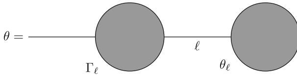
Fig. 13. The set \Gamma_\ell = \Gamma_\ell(\theta) and the subtree \theta_\ell determined by the line \ell \in L(\theta) . If \ell is the root line then \Gamma_\ell = \emptyset
