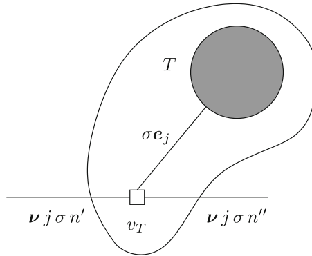
Fig. 10. A self-energy cluster in \mathfrak{E}_{j,\sigma,j,\sigma}^k(\omega \cdot \mathbf{v}, n) ; T contains at least one line on scale \leq n and n such that \min\{n', n''\} \geq n + 2
