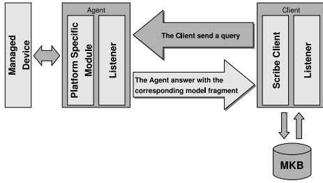
Fig. 4. A detailed view of the interaction between Agent and Client.
