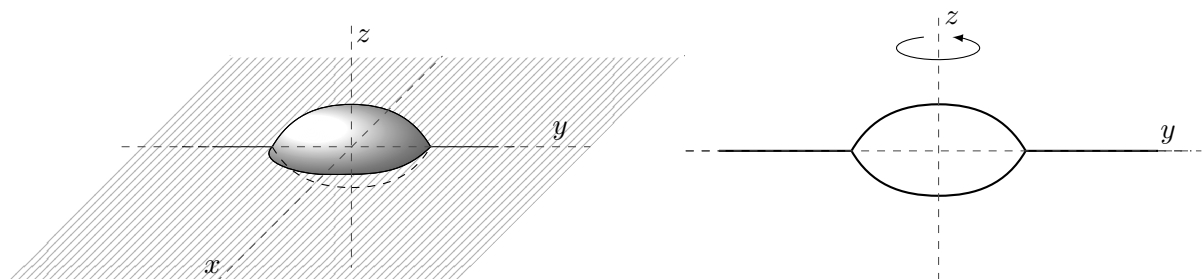
Figure 2: A rotationally symmetric “lens shaped” cluster.
