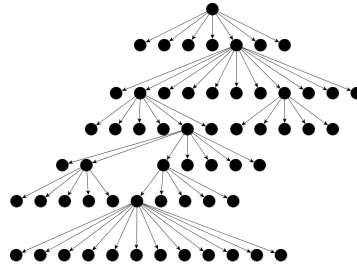
Figure 3.11: GUI Tree inferred by T4
