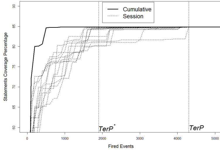
Figure 6.5: Two termination points of TP22 execution
