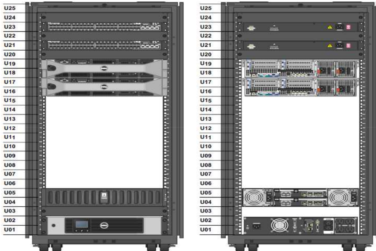
25U rack: front-rear view
