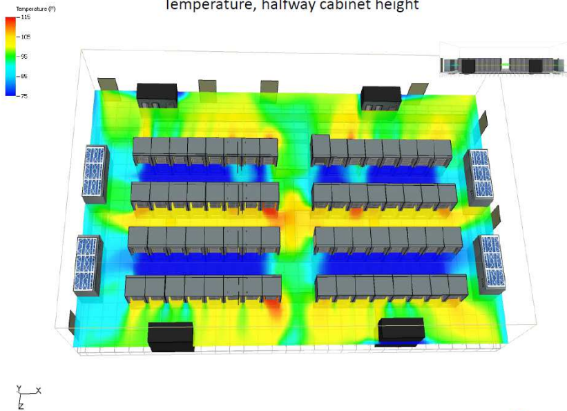
Standard (Hot Aisle/Cold Aisle)
