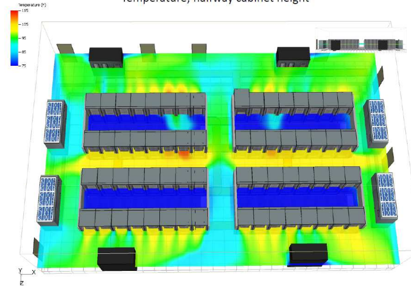
Standard Cold Aisle Containment
