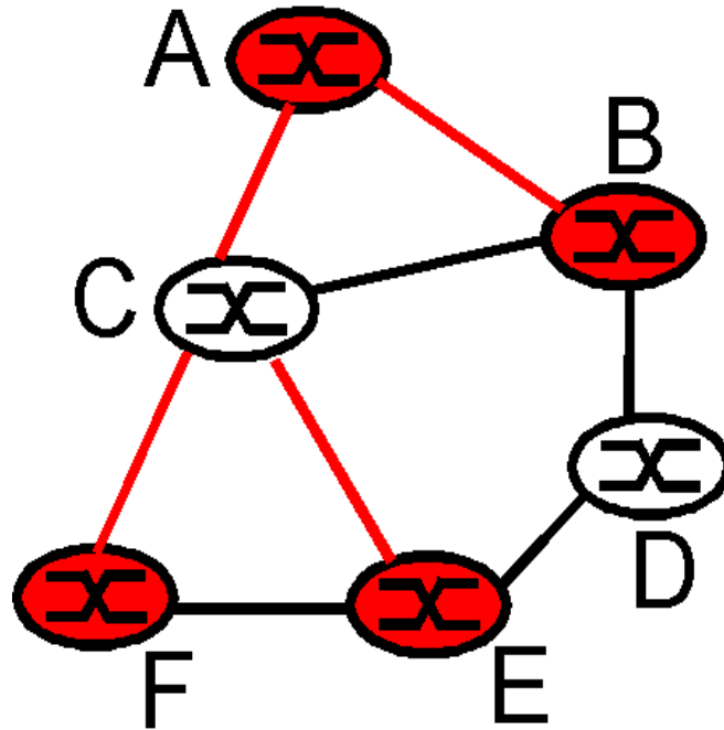
Group-shared Tree
