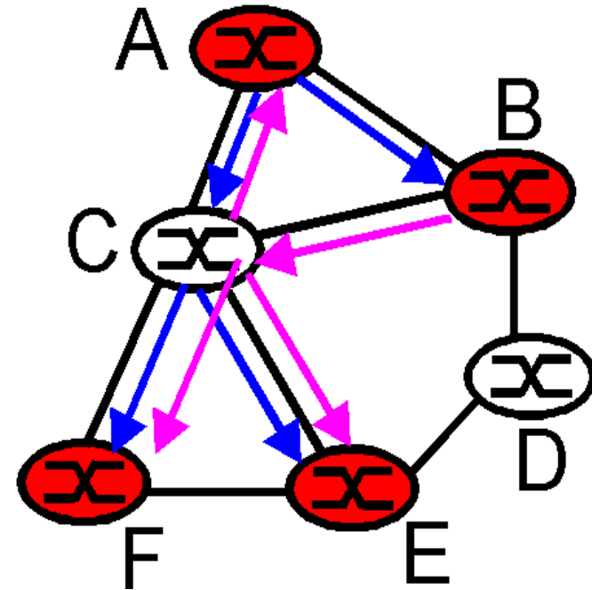
Source-based Tree
