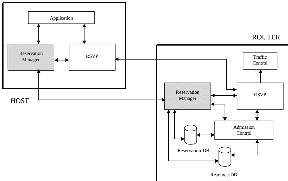
Figure 1: Hosts and routers structure
