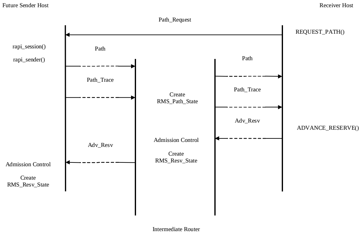
Figure 3: Typical handshaking for the negotiation phase of an Advance Reservation
