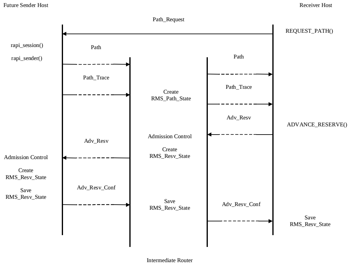
Figure 4: Confirmation message for advance reservations
