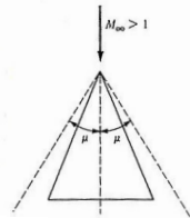
Subsonic leading edge
