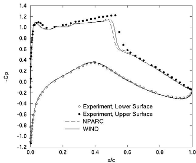
Pressure coefficient on the airfoil.
