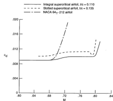
Variation of section drag coefficient with Mach number for section normal-force coefficient of 0.65.
