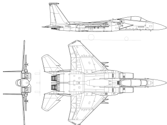
Area rule applied to F-15A
