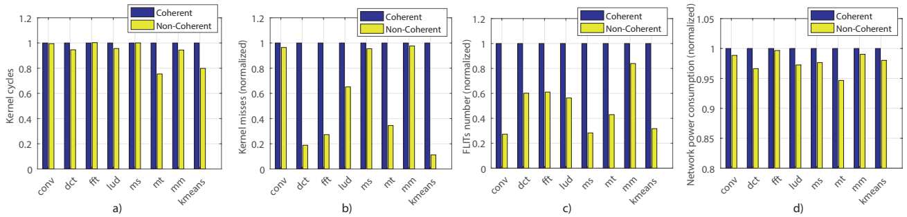
Fig. 2. a) Number of cycles for each kernel in coherent and noncoherent configurations. b) Total number of data misses in the whole system. c) Total number of flits flowing through the network-on-chip. d) Dynamic power consumption of the networking infrastructure.
