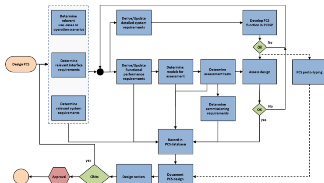
Figure 1. Flow diagram of the ITER PCS design process
