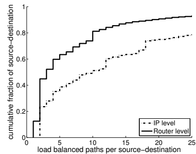
Figure 1: Overestimation of load balanced paths.
